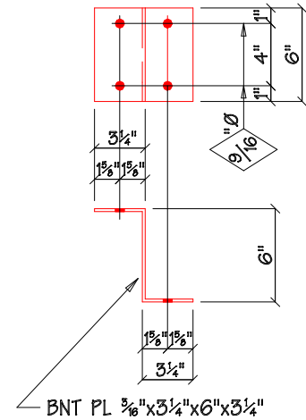
EW COLUMN CLIP~MK P11
