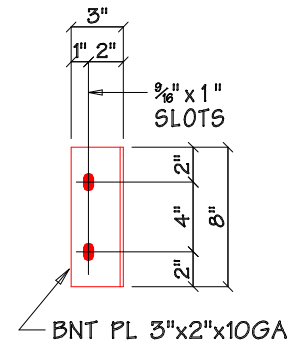
PURLIN CLIP~MK P4
