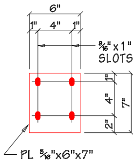
PURLIN & GIRT CLIP~MK P1
