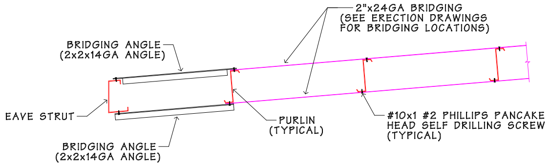
SECTION AT ROOF BRIDGING
