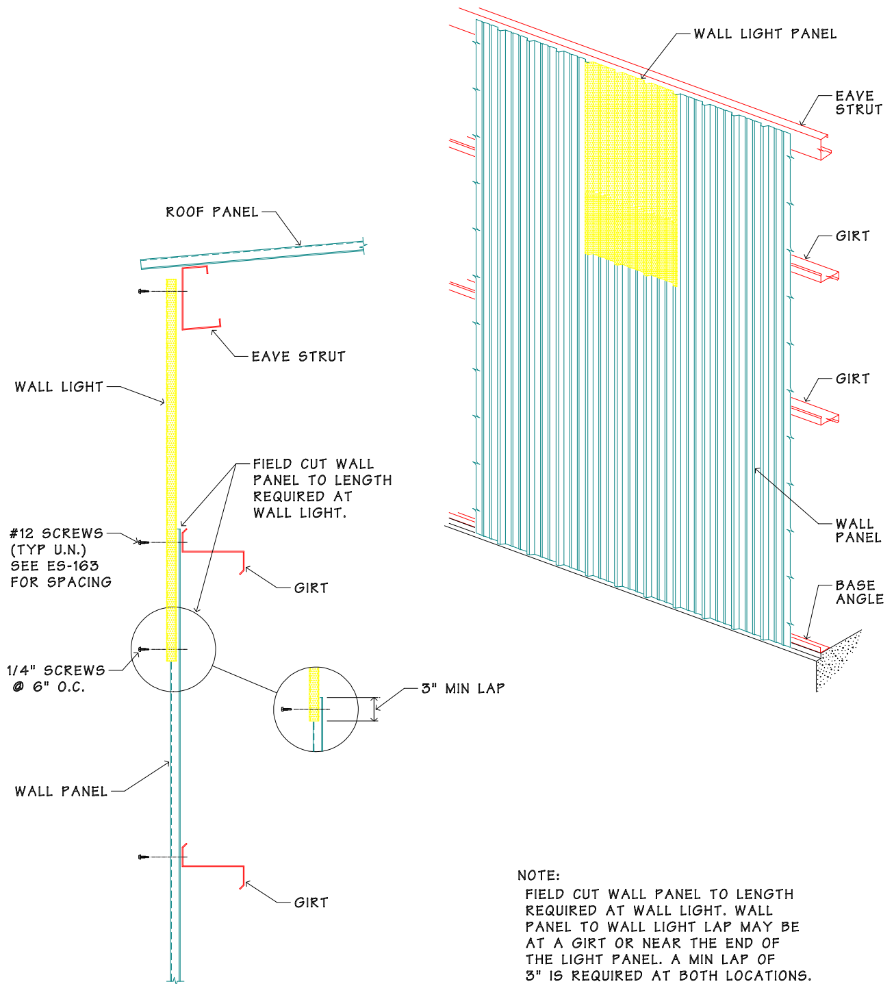
VERTICAL SECTION THRU WALL LIGHT
