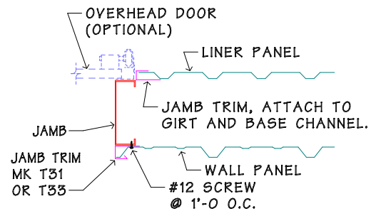
SECTION THRU JAMB WITH LINER PANEL
