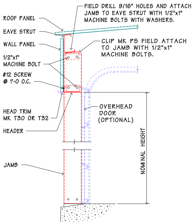
VERTICAL SECTION THRU DOOR OPENING AT SIDEWALL
