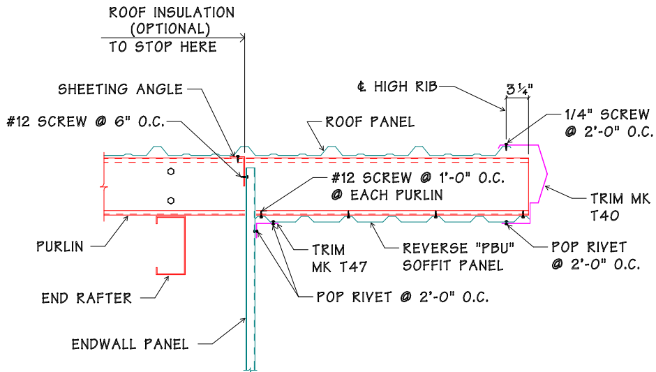
TYPICAL SECTION THRU PURLIN EXTENSION
