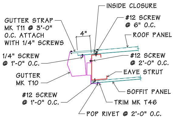
SECTION AT GUTTER
