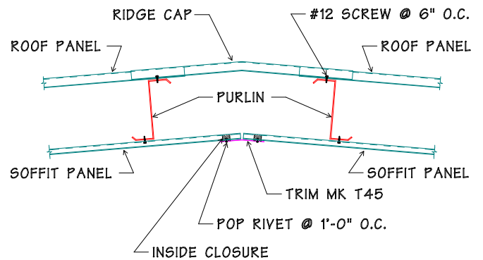
SECTION AT RIDGE
