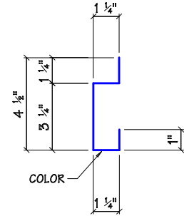
GUTTER STANDOFF - MK T12
