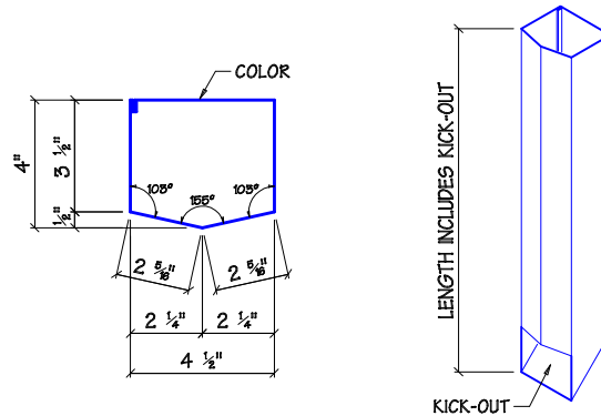
GUTTER DOWNSPOUT - MK T14
