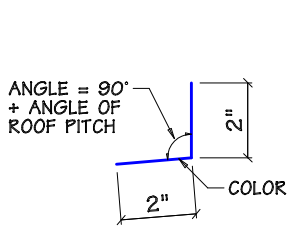
EAVE EXT TRIM - MK T38
