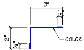
PURLIN EXT TRIM - MK T47
