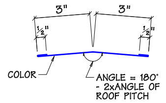
PURLIN EXT TRIM - MK T45
