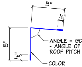
EAVE EXT TRIM - MK T43
