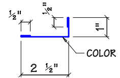
SKYLIGHT TRIM - MK T50
