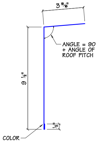
EAVE EXT TRIM - MK T44
