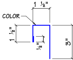
PANEL CAP TRIM - MK T48 ( "R" PANEL )
