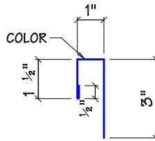
PANEL CAP TRIM - MK T49 ( "U" PANEL )
