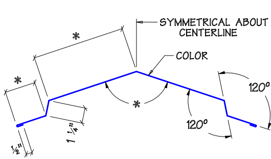
"SS" RIDGE FLASH - MK T59 (FOR USE WITHOUT RIDGE VENTS)
