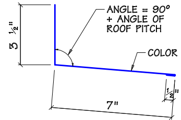
LEAN-TO FLASHING - MK T70
