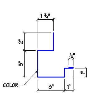
FASCIA NOSE TRIM - MK T110
