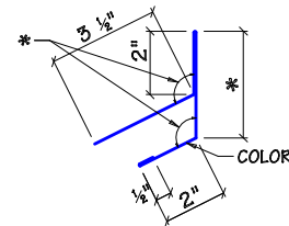
EAVE EXTENSION TRIM - MK T152 "REV U" SOFFIT PANEL
