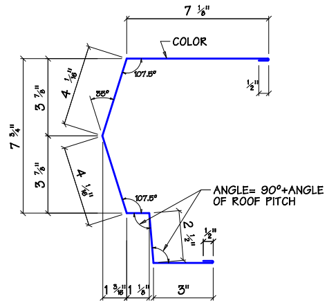
EAVE TRIM - MK T143
