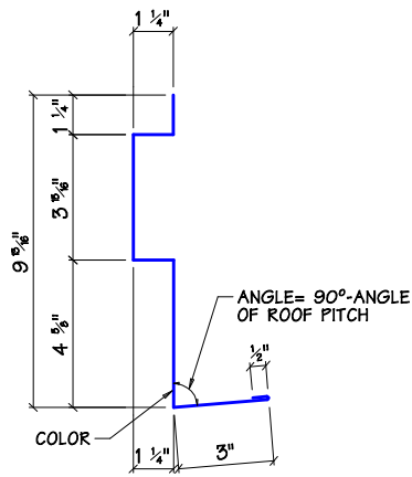
PURLIN EXTENSION TRIM - MK T141
