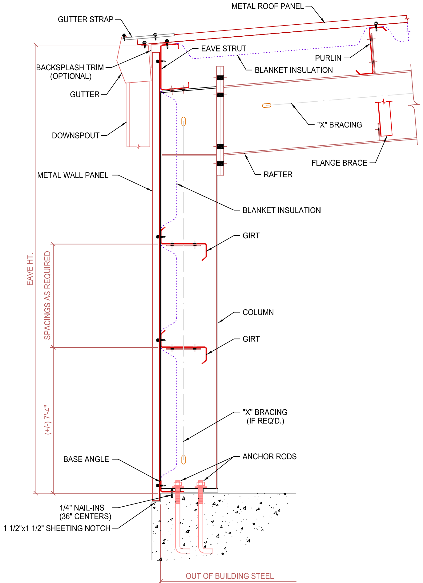
STANDARD SIDEWALL SECTION (FLUSH GIRT SYSTEM)
