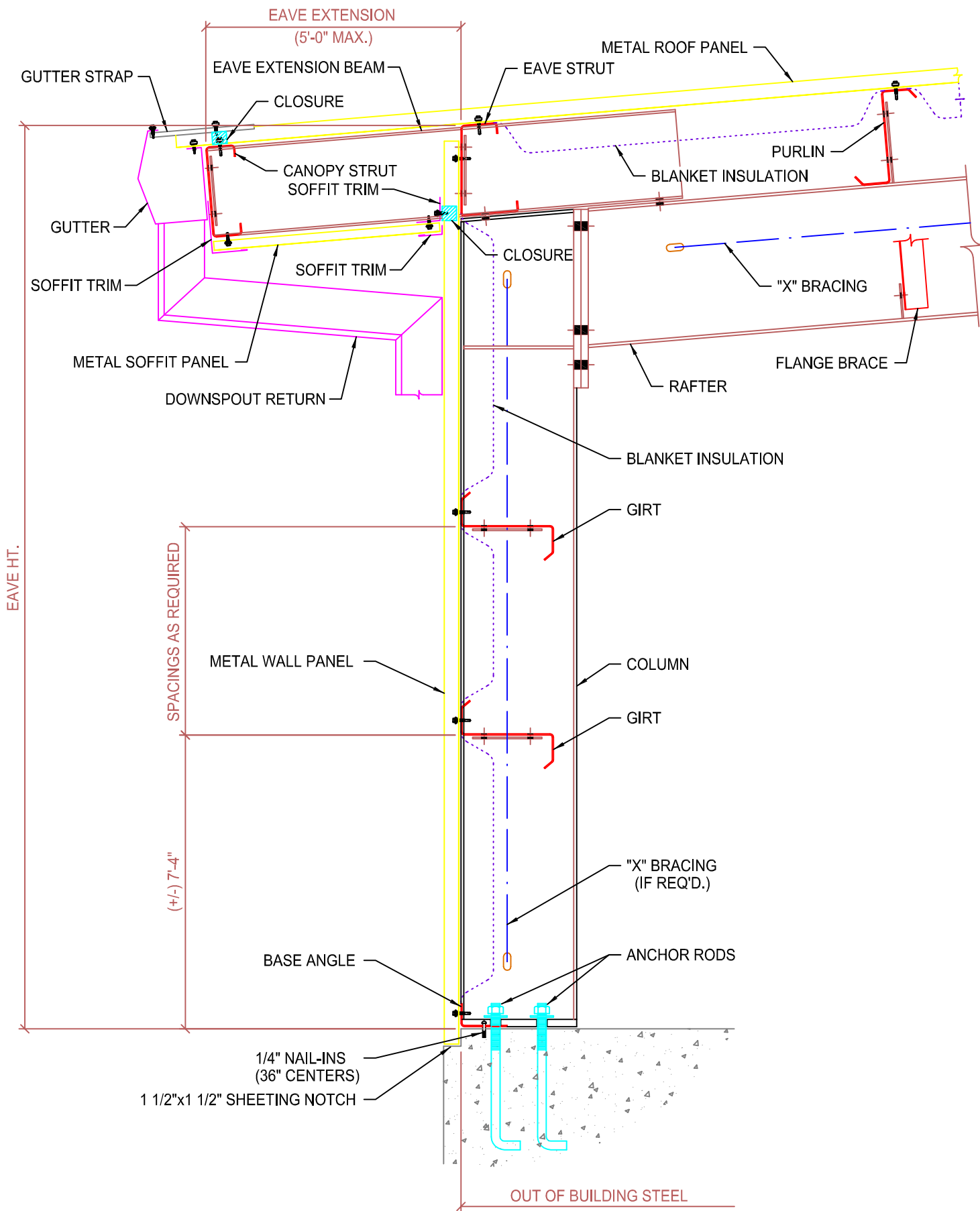
STANDARD SIDEWALL SECTION (FLUSH GIRTS SYSTEM) WITH EAVE EXTENSION
