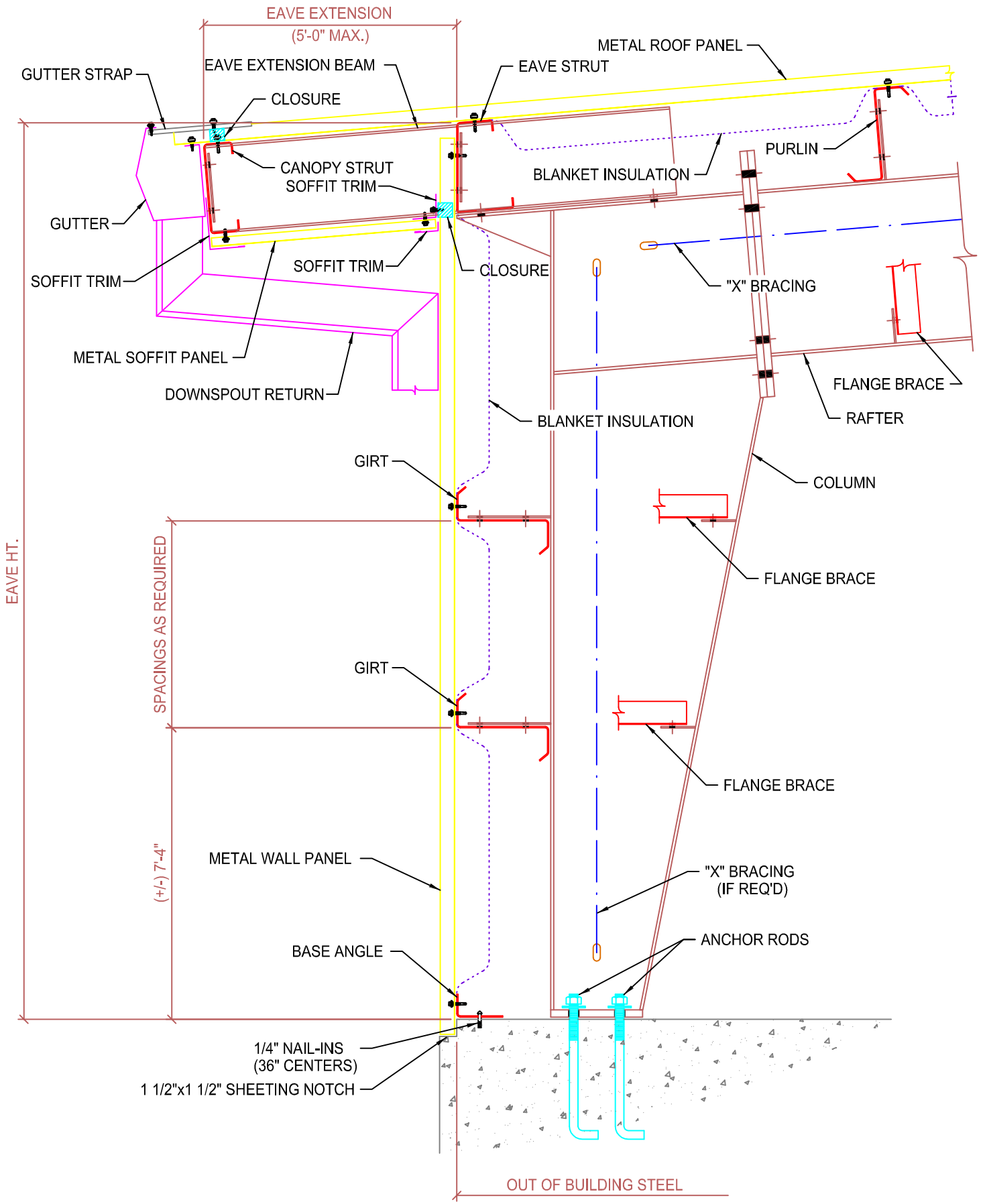
STANDARD SIDEWALL SECTION (BYPASS GIRT SYSTEM) WITH EAVE EXTENSION
