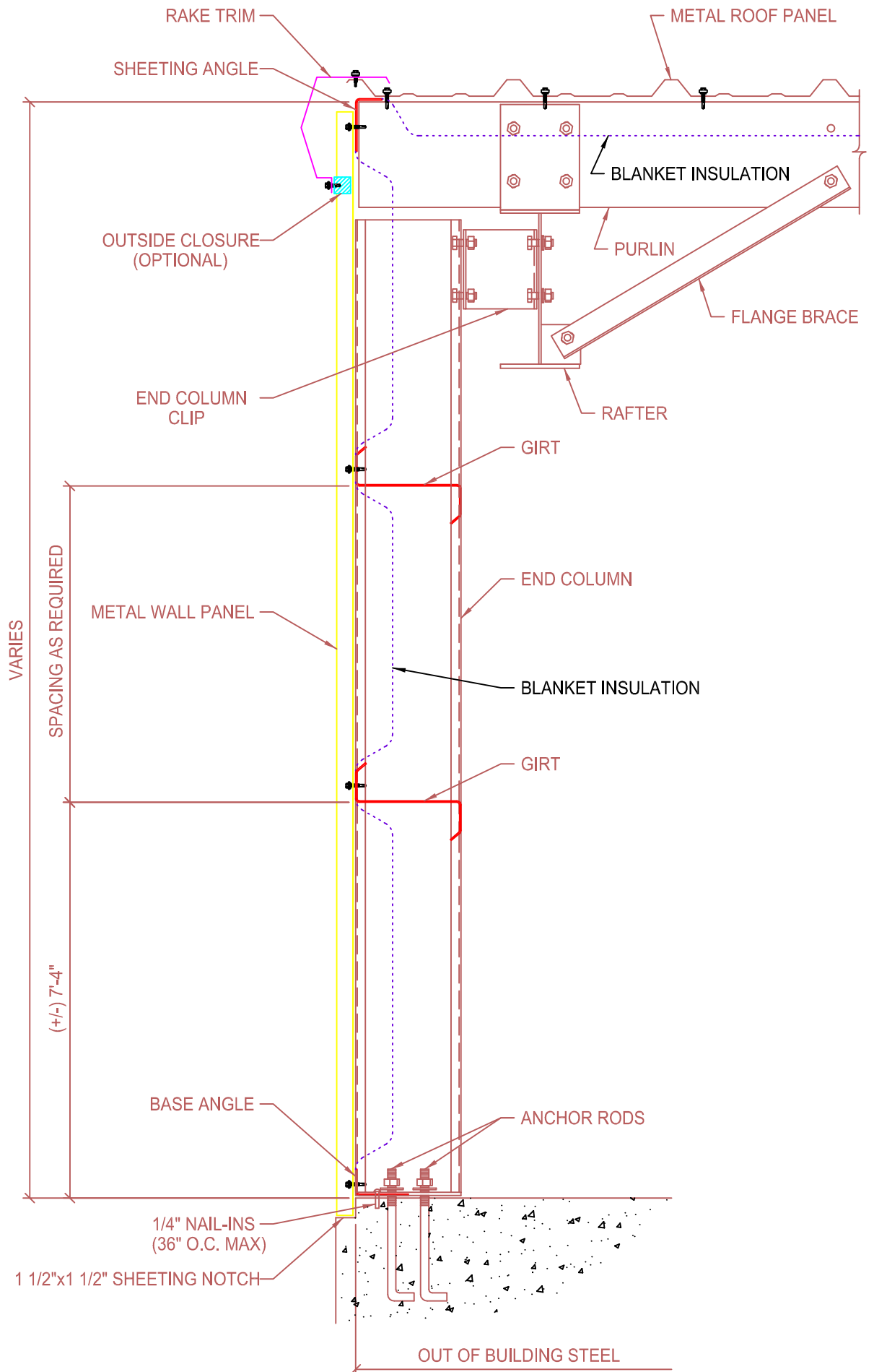
RIGID FRAME ENDWALL SECTION (FLUSH GIRT SYSTEM)
