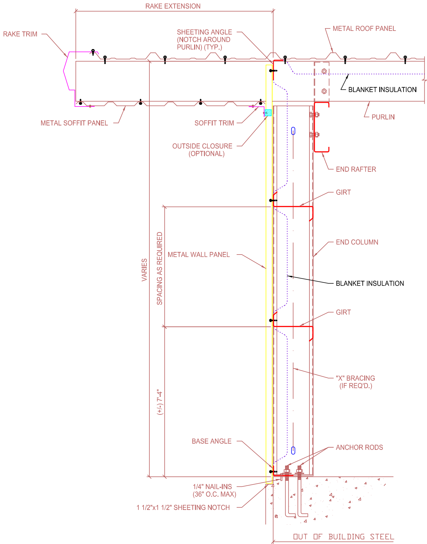
BEARING ENDWALL SECTION (FLUSH GIRTS SYSTEM) WITH RAKE EXTENSION
