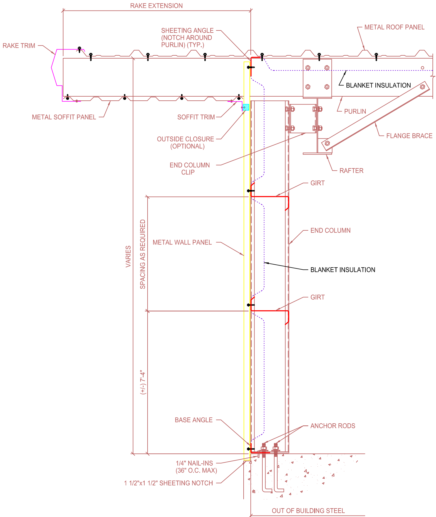
RIGID FRAME ENDWALL SECTION (FLUSH GIRT SYSTEM) WITH RAKE EXTENSION
