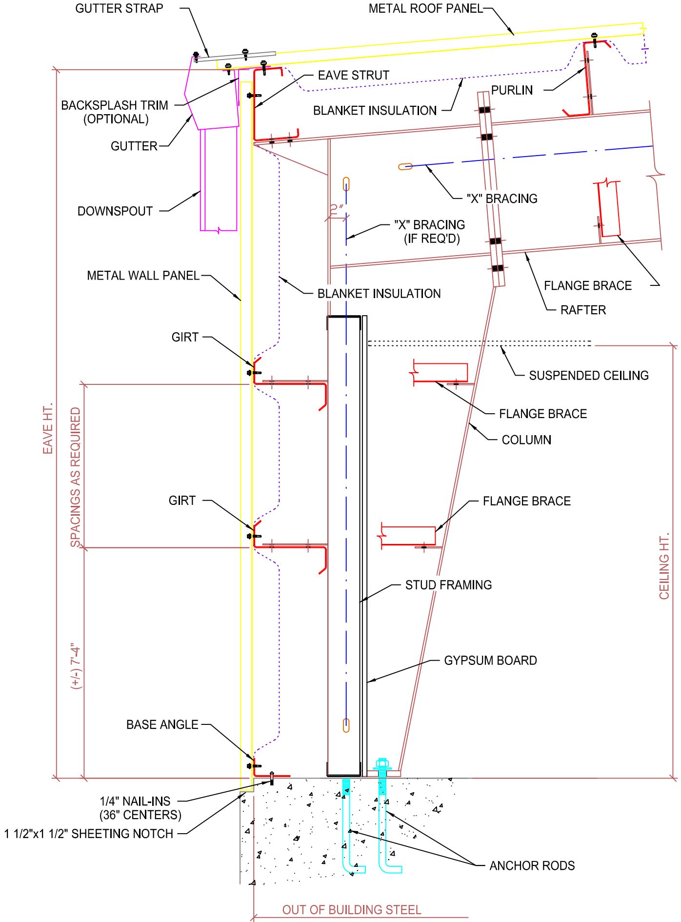
STANDARD SIDEWALL SECTION (BYPASS GIRT SYSTEM) WITH STUD WALLS
