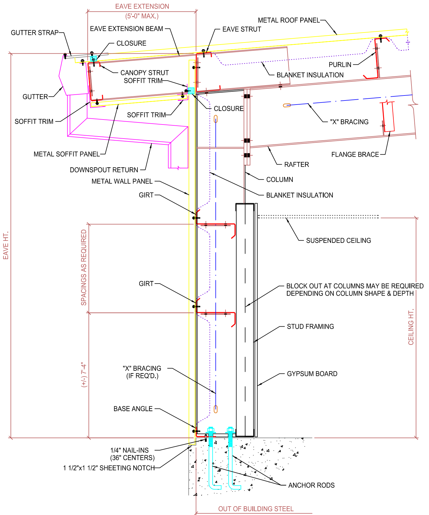
STANDARD SIDEWALL SECTION (FLUSH GIRTS SYSTEM) WITH EAVE EXTENSION & STUD WALLS
