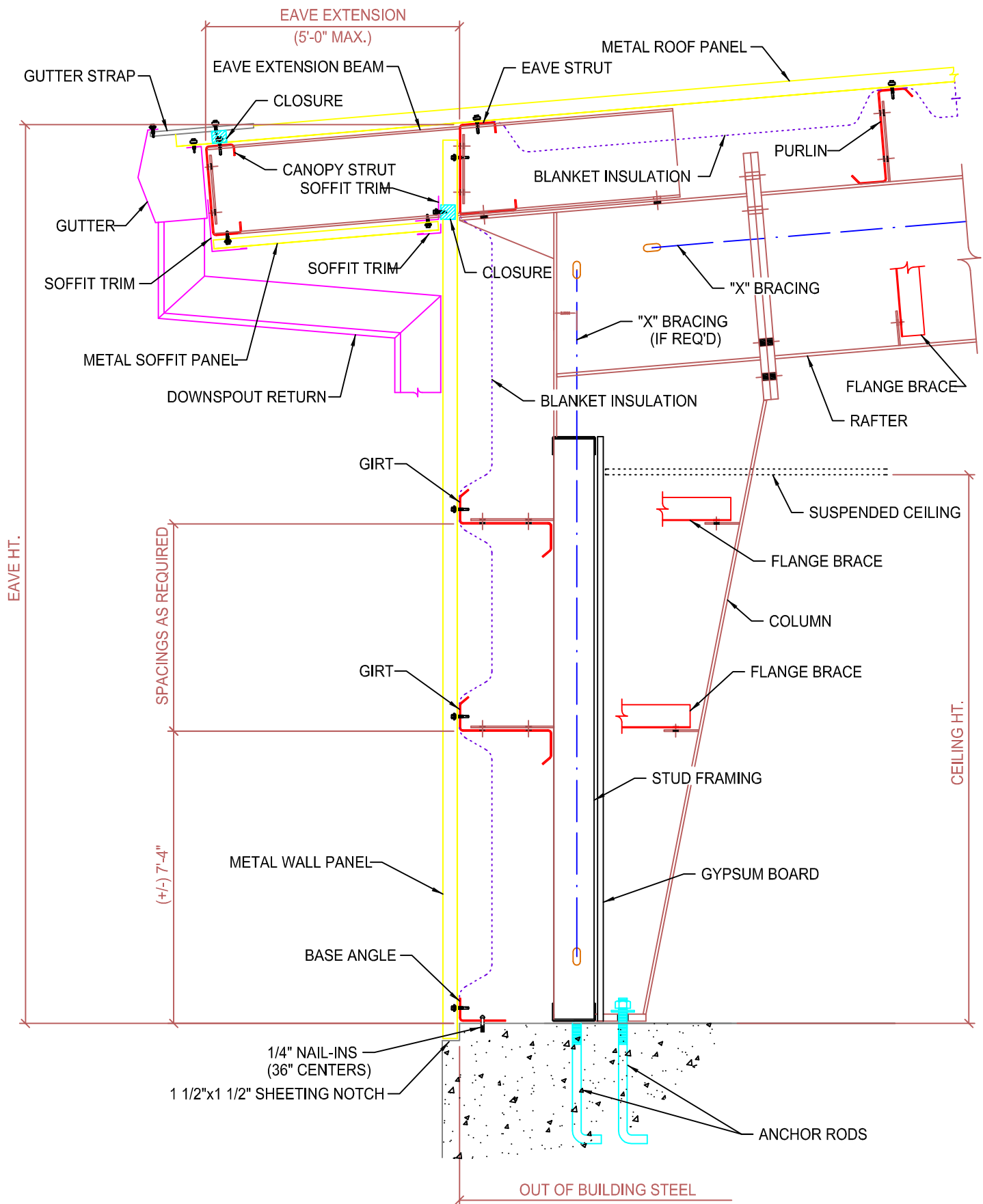
STANDARD SIDEWALL SECTION (BYPASS GIRTS SYSTEM) WITH EAVE EXTENSION & STUD WALLS
