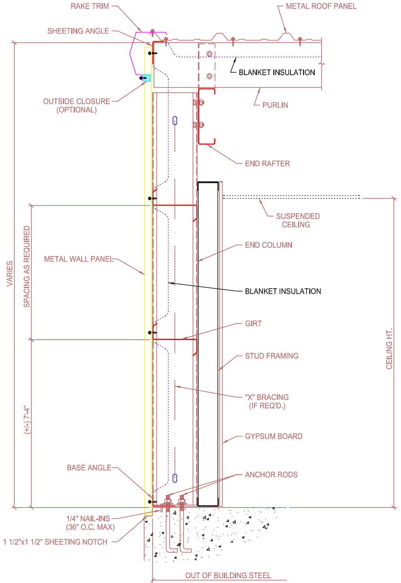
BEARING ENDWALL SECTION (FLUSH GIRT SYSTEM) WITH STUD WALLS
