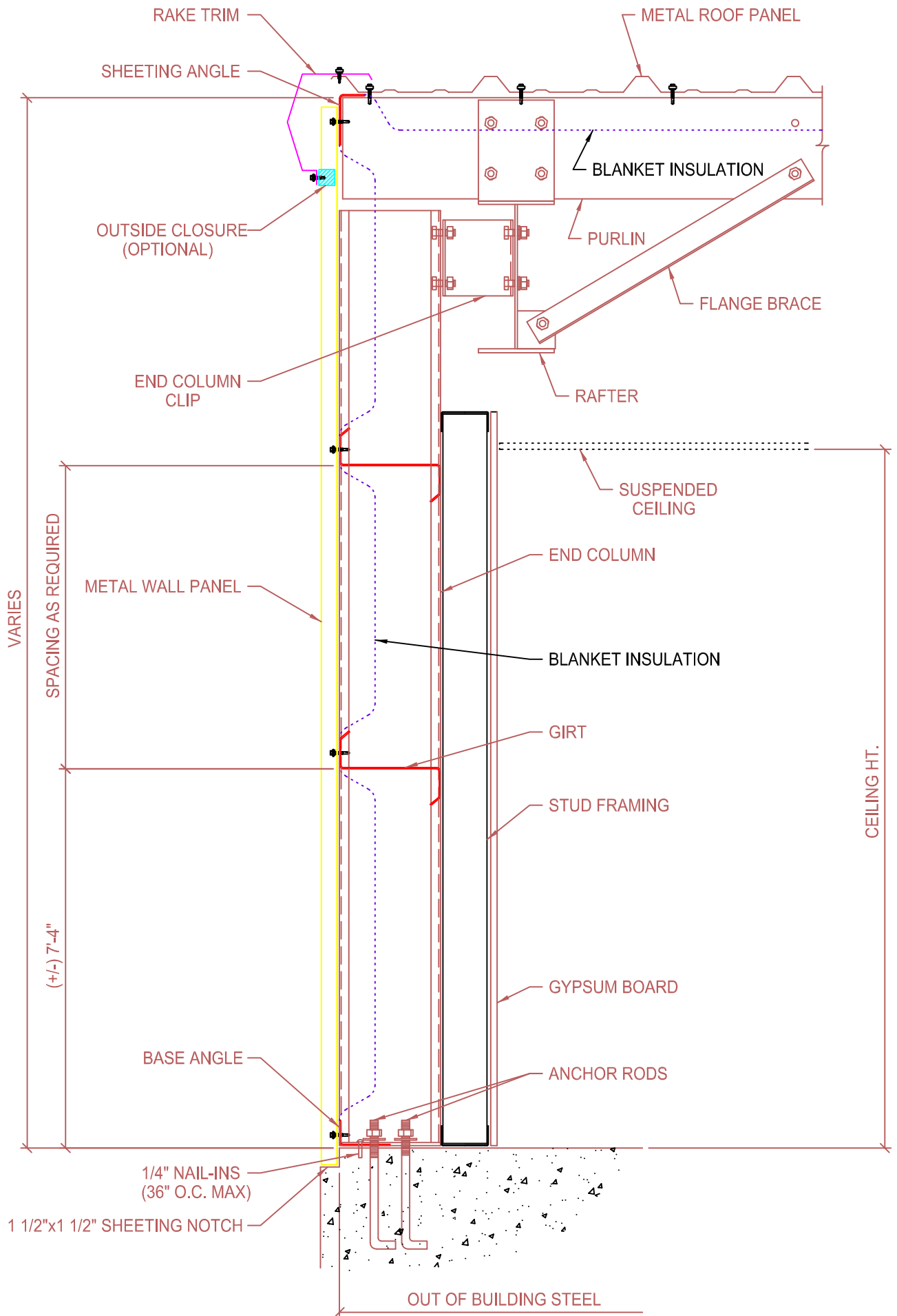
RIGID FRAME ENDWALL SECTION (FLUSH GIRT SYSTEM) WITH STUD WALLS
