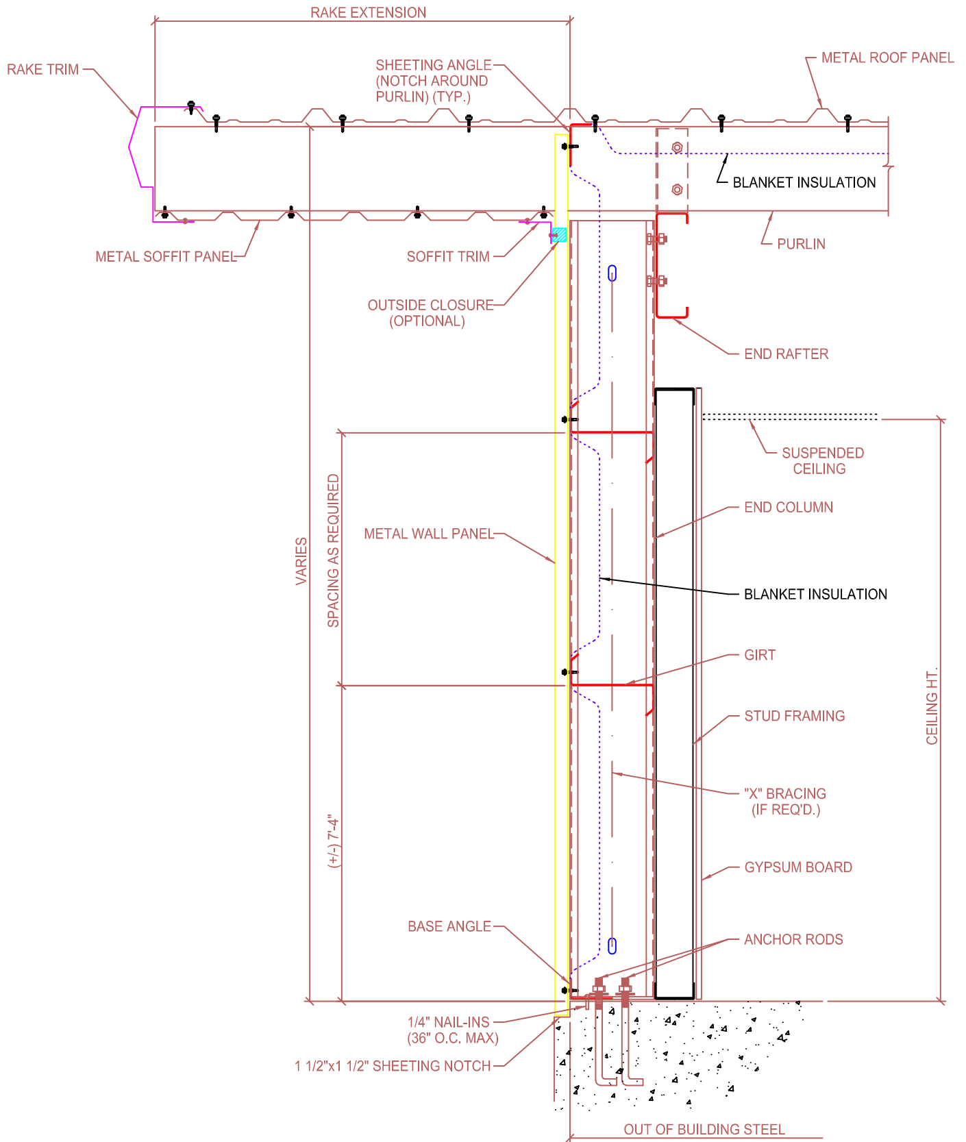
BEARING ENDWALL SECTION (FLUSH GIRT SYSTEM) WITH RAKE EXTENSION & STUD WALLS
