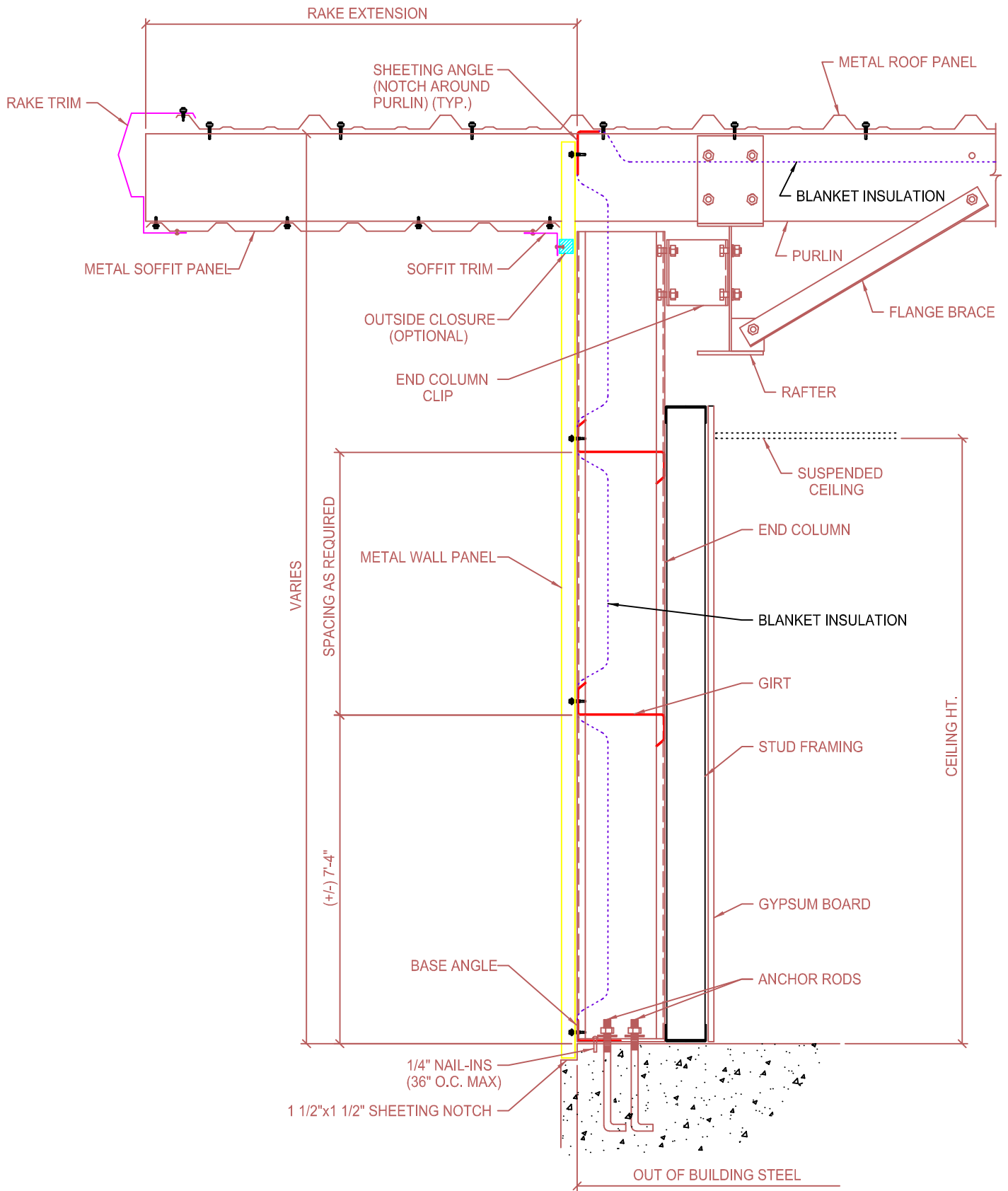
RIGID FRAME ENDWALL SECTION (FLUSH GIRTS SYSTEM) WITH RAKE EXTENSION & STUD WALLS
