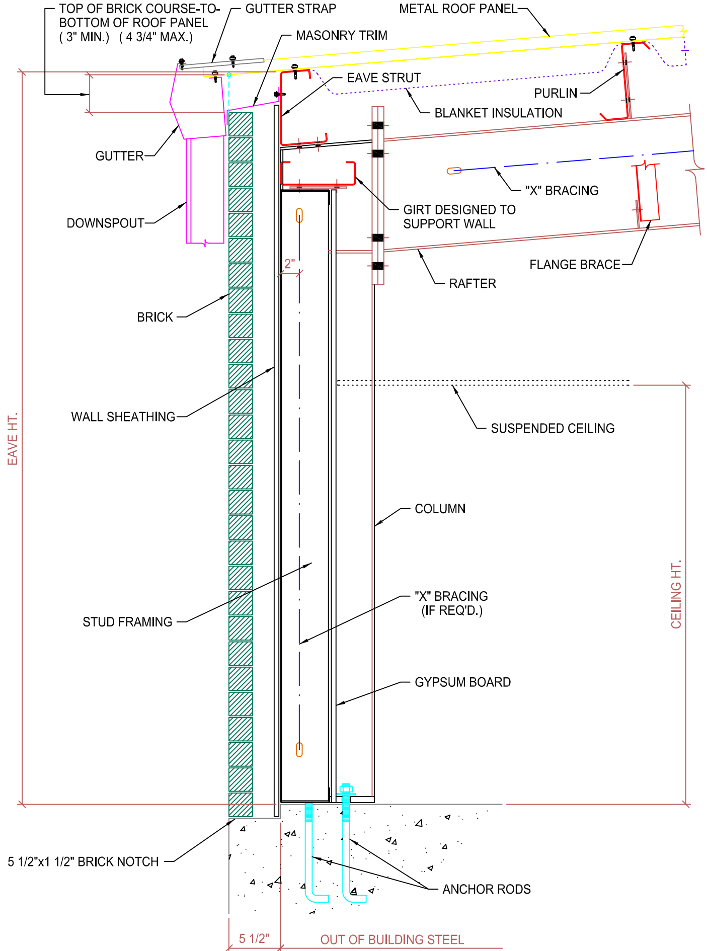
SIDEWALL SECTION OPEN FOR WALL MATERIAL BY OTHERS (FLUSH GIRTS SYSTEM)
