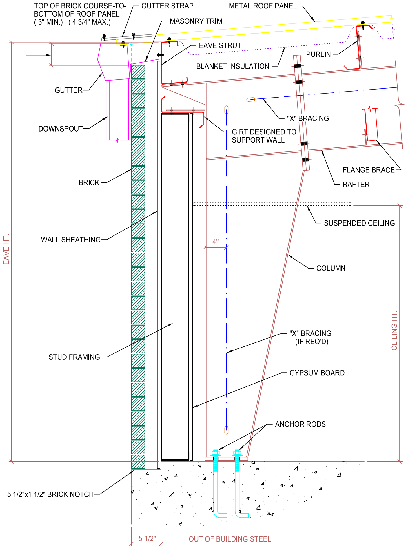
SIDEWALL SECTION OPEN FOR WALL MATERIAL BY OTHERS (BYPASS GIRTS SYSTEM)
