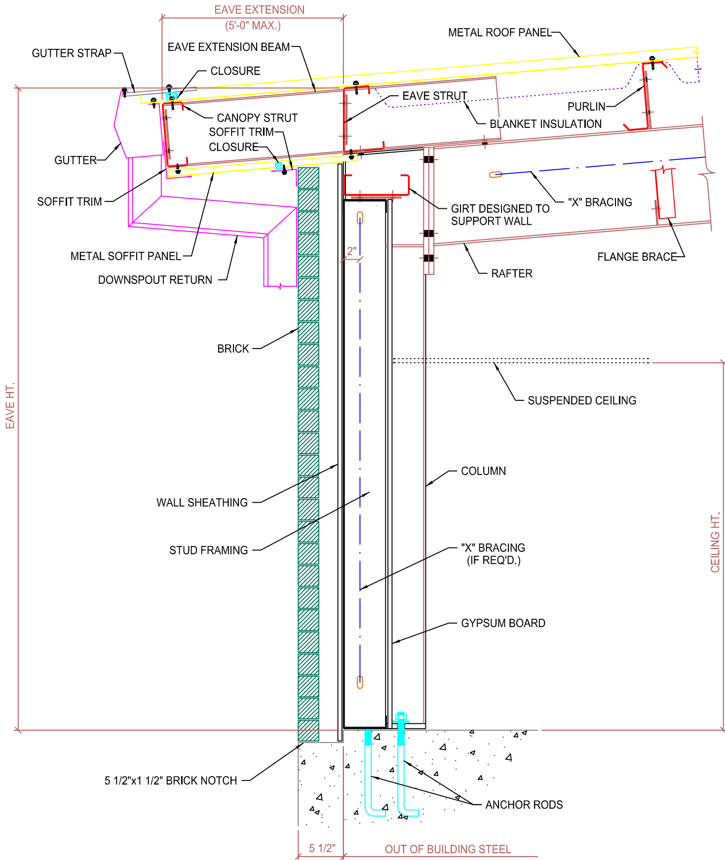
SIDEWALL SECTION OPEN FOR WALL MATERIAL BY OTHERS (FLUSH GIRT SYSTEM) (EAVE EXTENSION)
