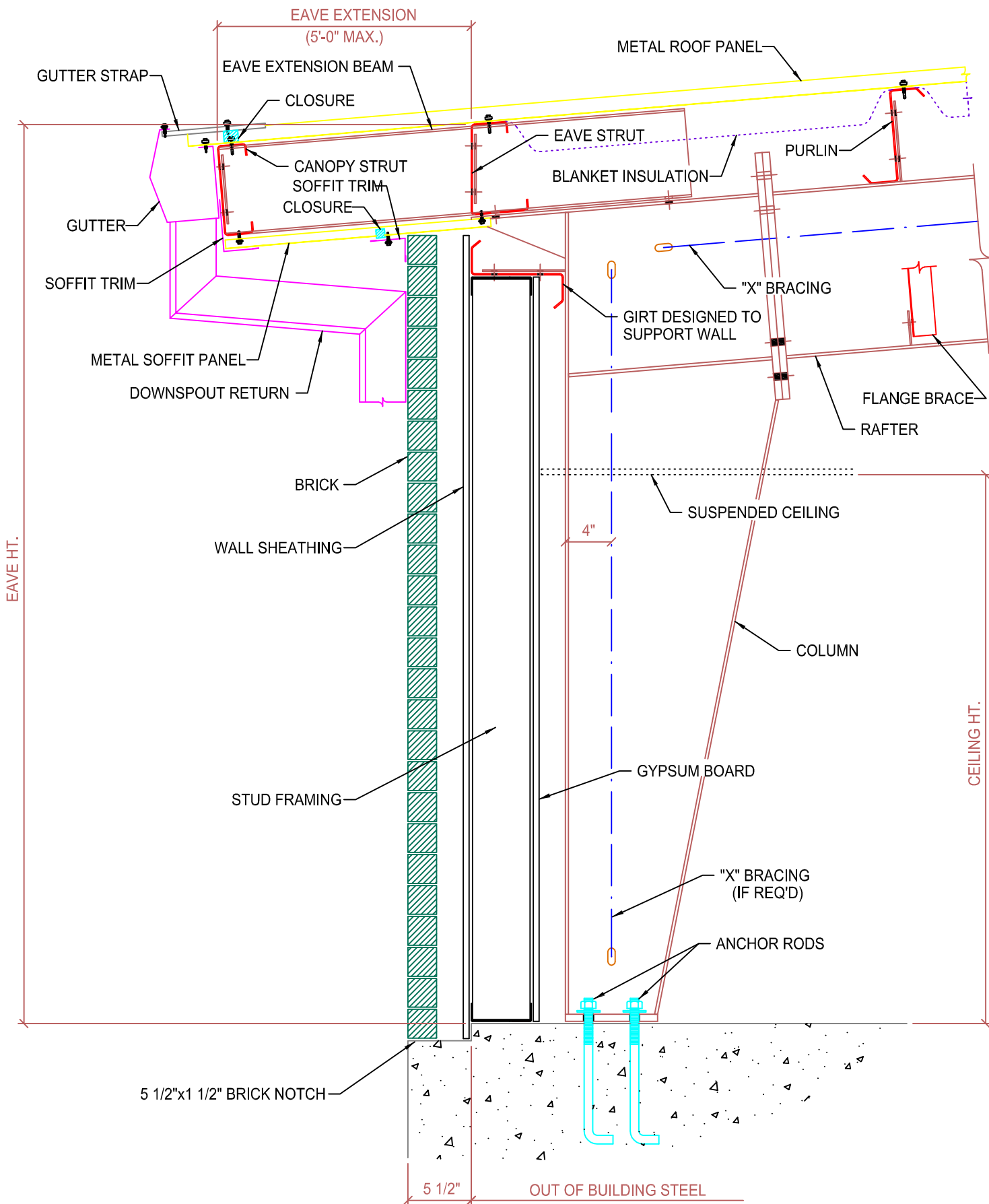
SIDEWALL SECTION OPEN FOR WALL MATERIAL BY OTHERS (BYPASS GIRTS SYSTEM) (EAVE EXTENSION)
