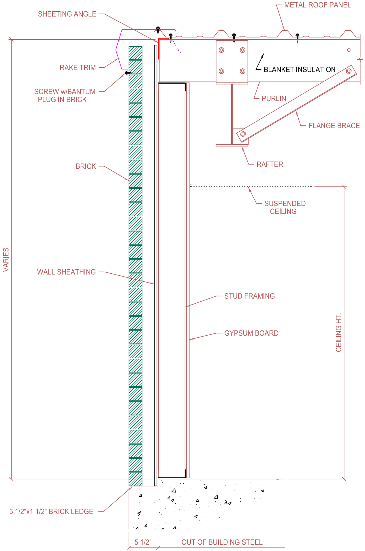
RIGID FRAME ENDWALL SECTION OPEN FOR WALL MATERIAL BY OTHERS
