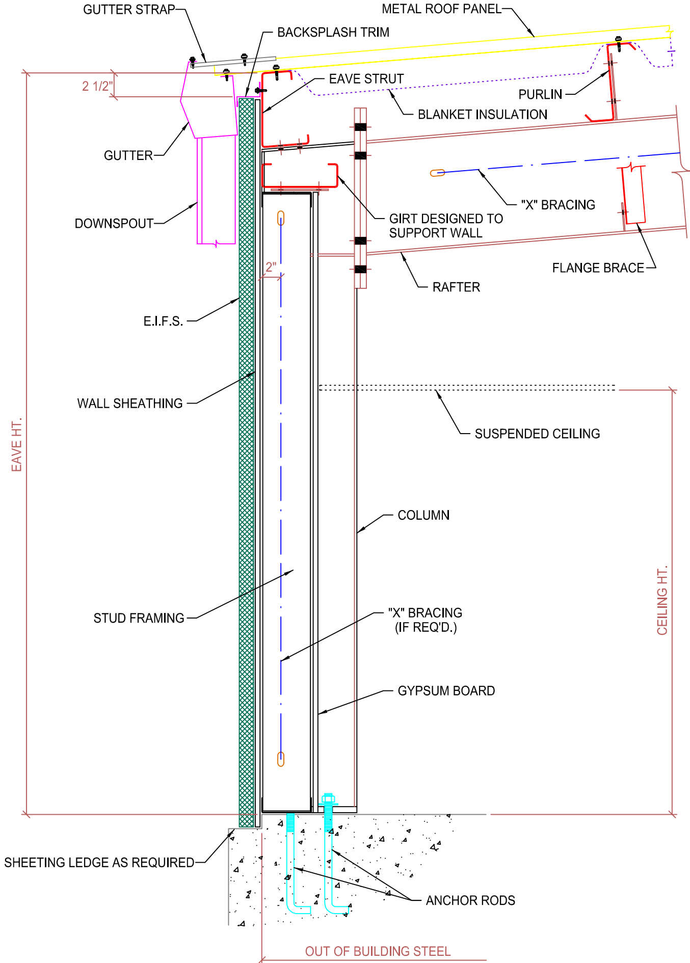
SIDEWALL SECTION OPEN FOR WALL MATERIAL BY OTHERS (FLUSH GIRT SYSTEM)
