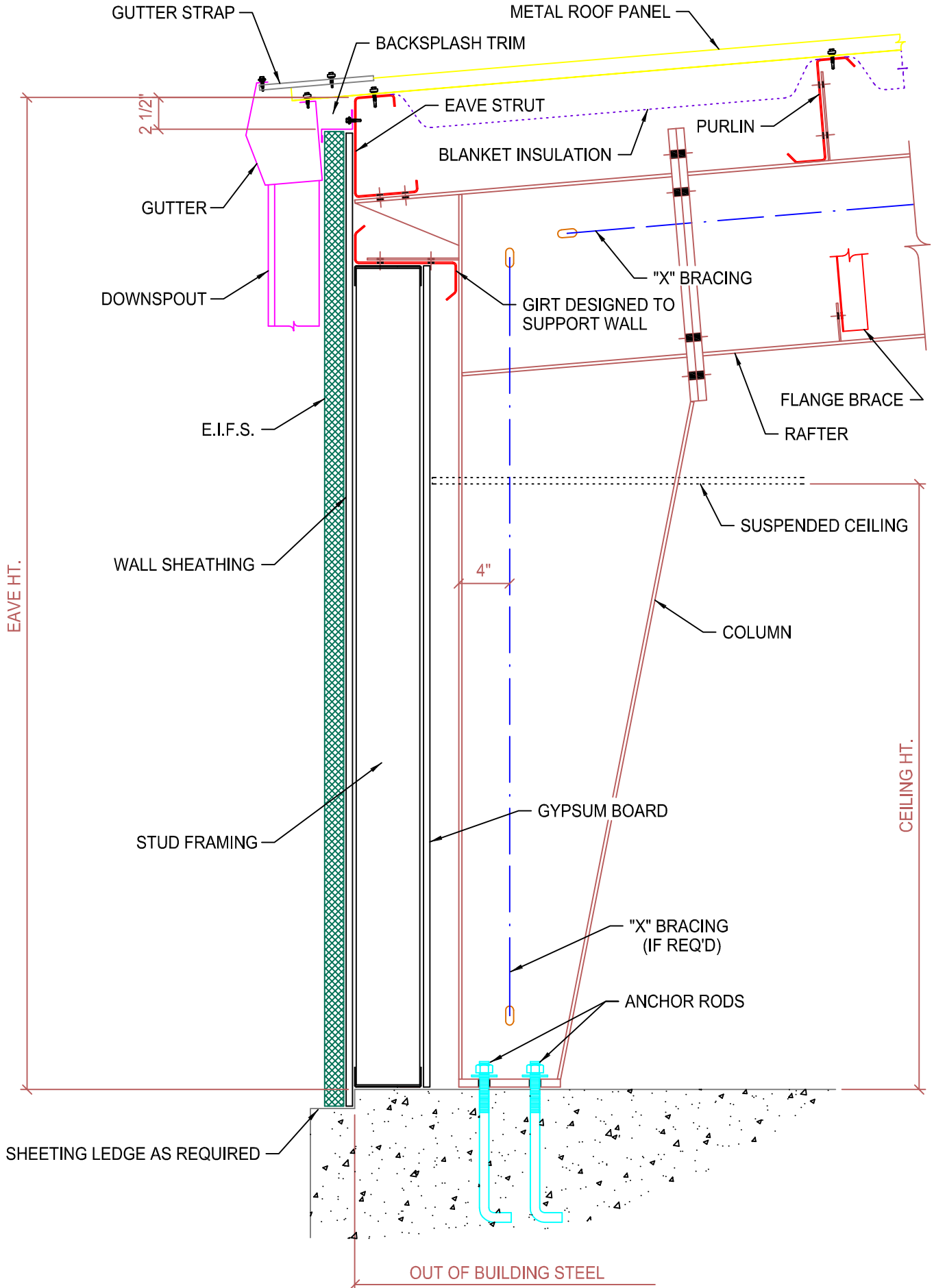
SIDEWALL SECTION OPEN FOR WALL MATERIAL BY OTHERS (BYPASS GIRT SYSTEM)
