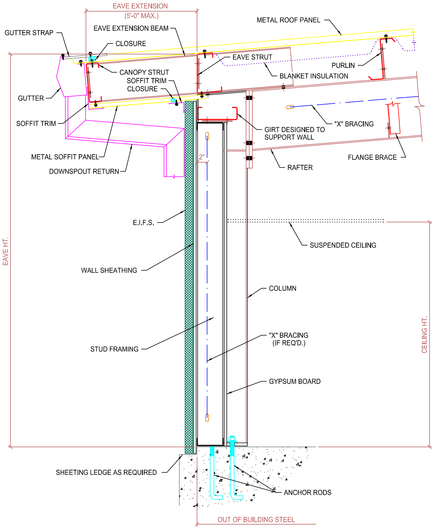
SIDEWALL SECTION OPEN FOR WALL MATERIAL BY OTHERS (FLUSH GIRT SYSTEM) (EAVE EXTENSION)
