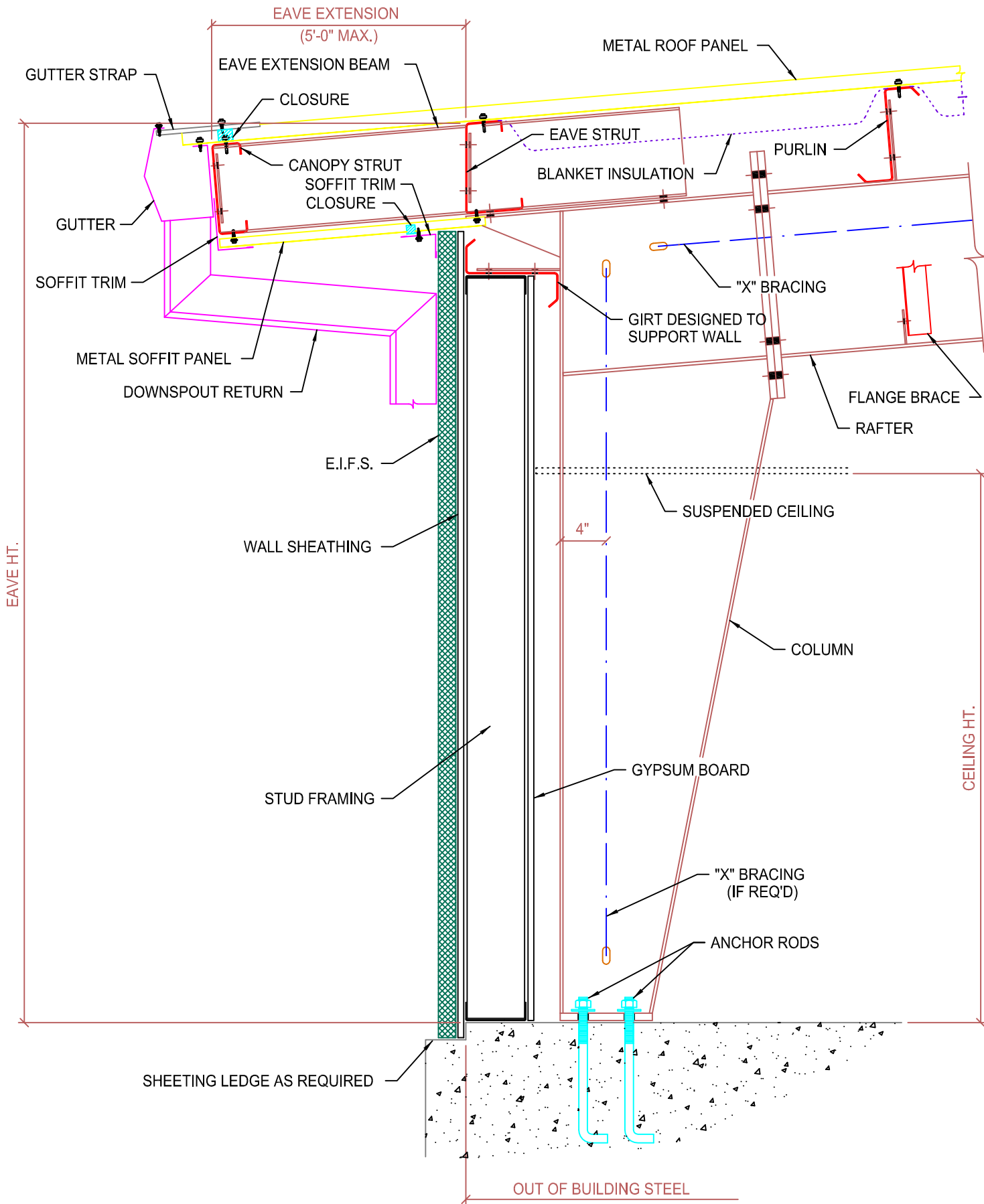
SIDEWALL SECTION OPEN FOR WALL MATERIAL BY OTHERS (BYPASS GIRT SYSTEM) (EAVE EXTENSION)
