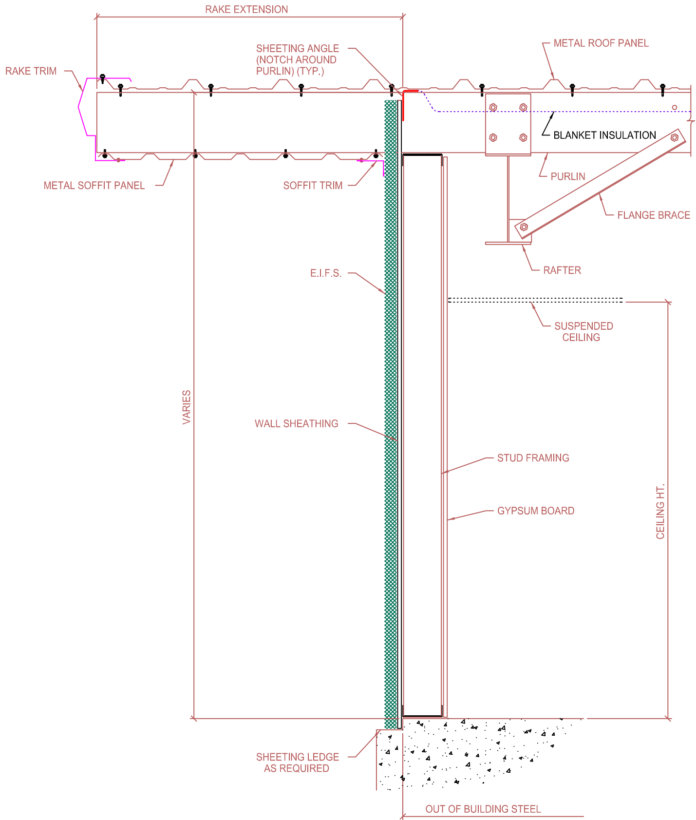
RIGID FRAME ENDWALL SECTION OPEN FOR WALL MATERIAL BY OTHERS WITH RAKE EXTENSION
