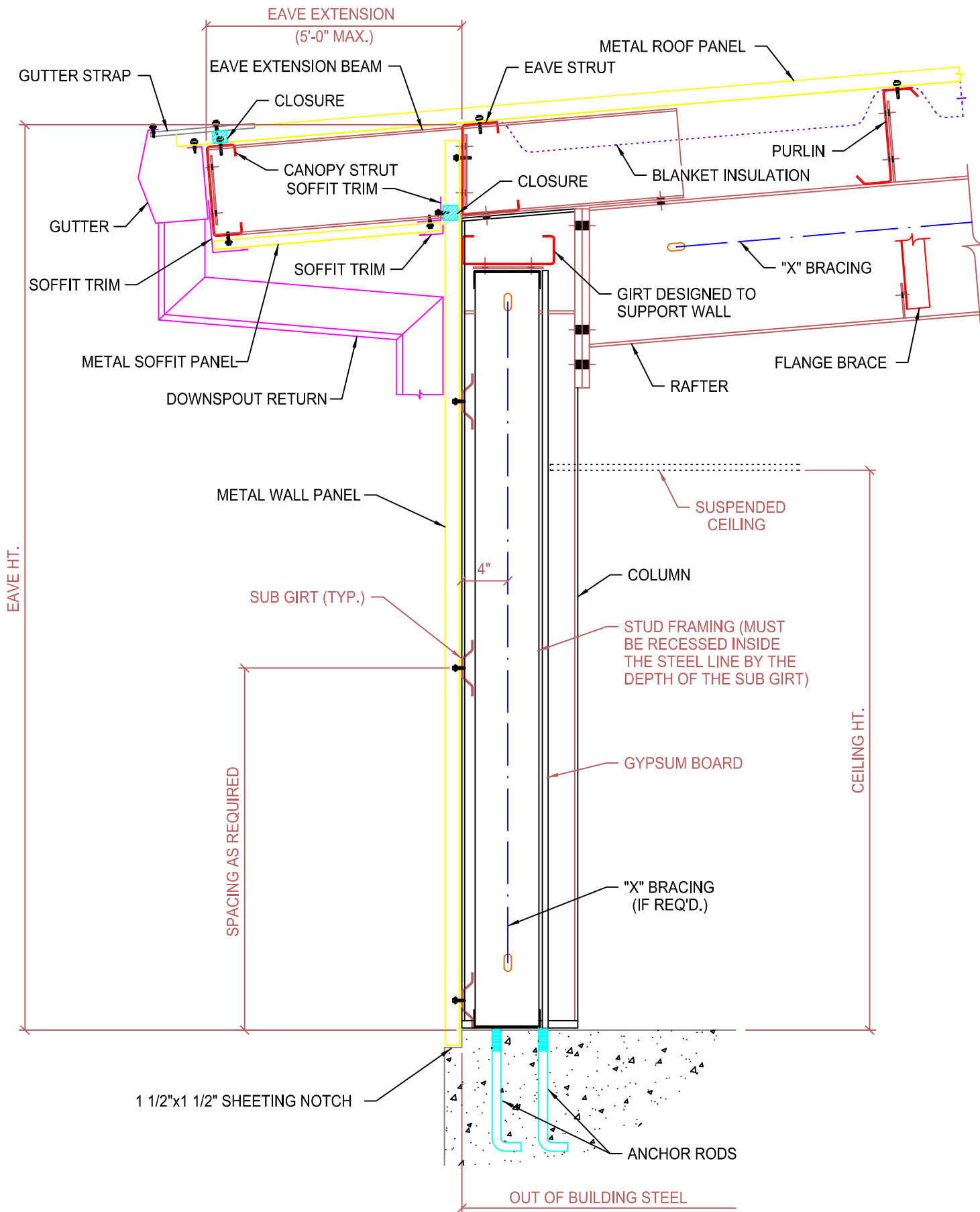
SIDEWALL SECTION OPEN FOR WALL MATERIAL BY OTHERS WITH WALL PANELS AND EAVE EXTENSION
