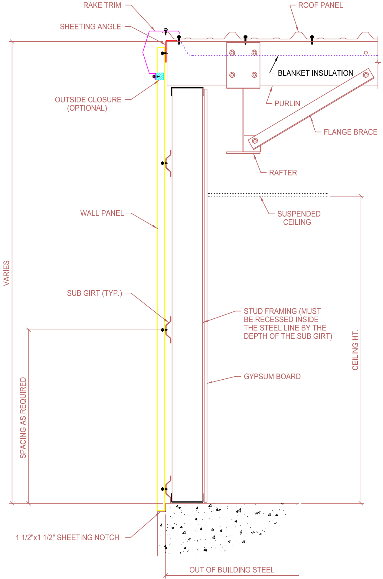
RIGID FRAME ENDWALL SECTION OPEN FOR WALL MATERIAL BY OTHERS WITH WALL PANELS
