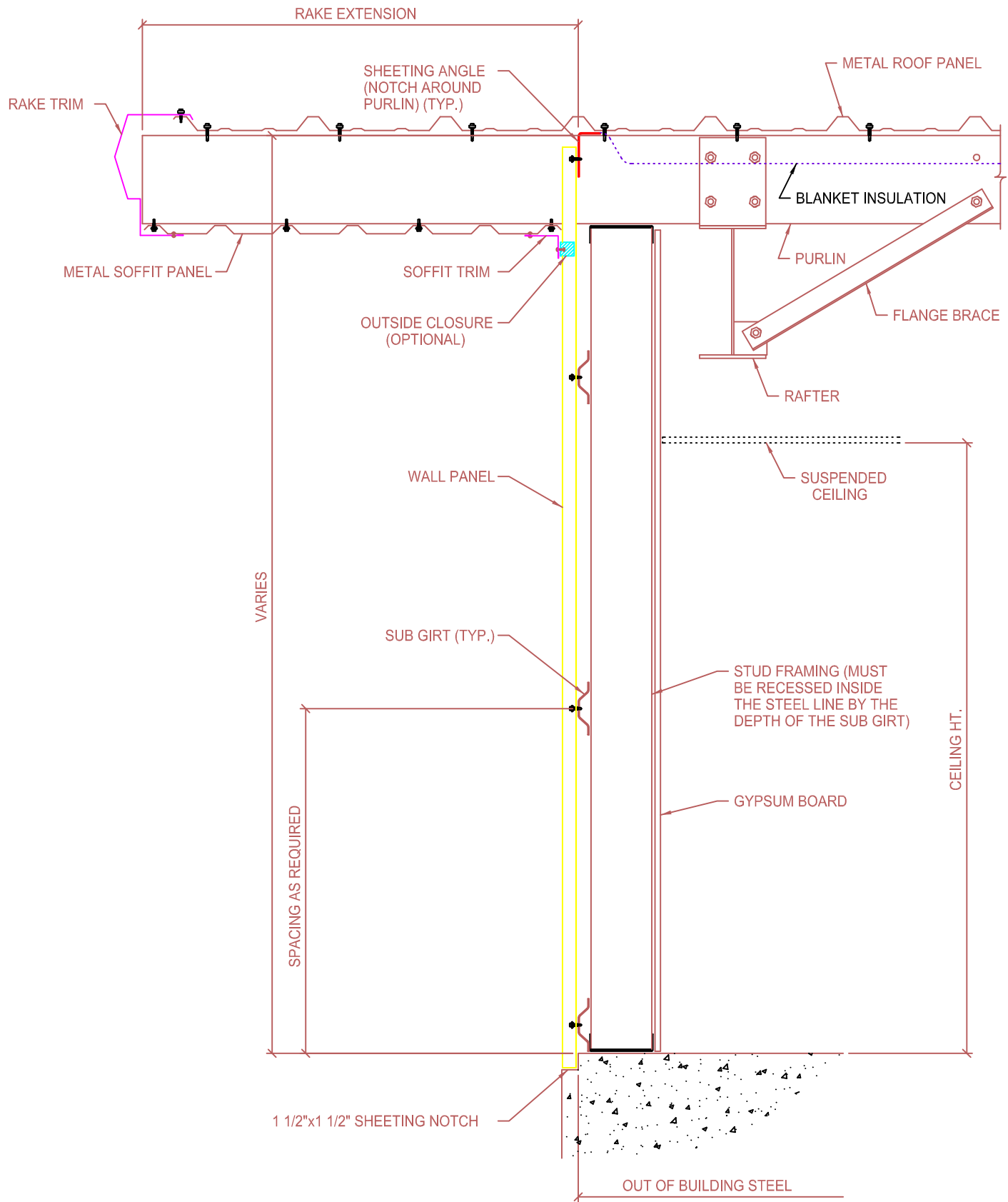
RIGID FRAME ENDWALL SECTION OPEN FOR WALL MATERIAL BY OTHERS WITH RAKE EXTENSION & WITH WALL PANELS
