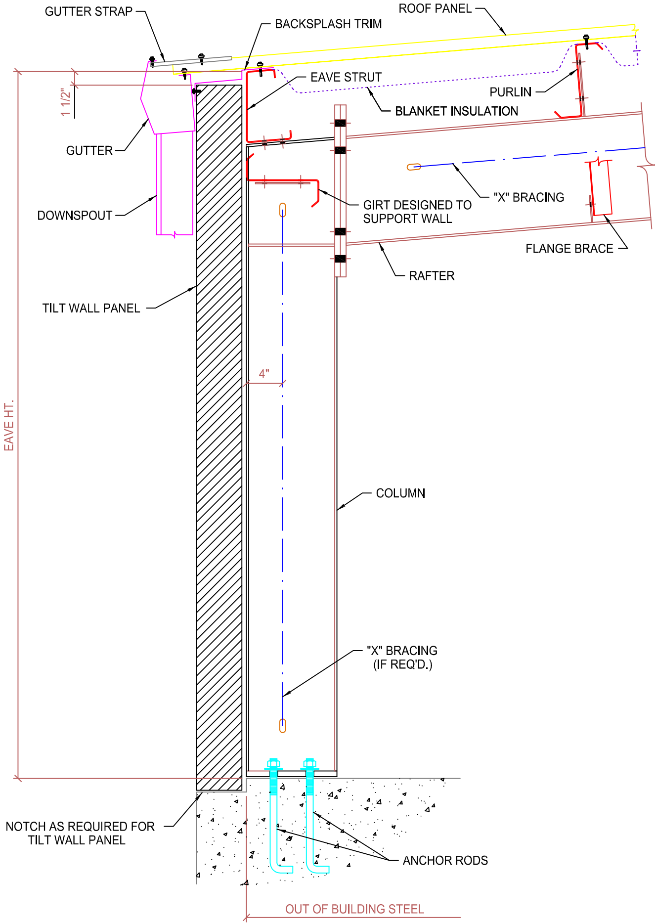
SIDEWALL SECTION OPEN FOR TILT WALL (FLUSH GIRT SYSTEM)
