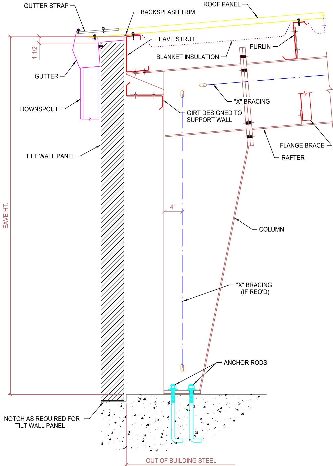
SIDEWALL SECTION OPEN FOR TILT WALL (BYPASS GIRTS SYSTEM)
