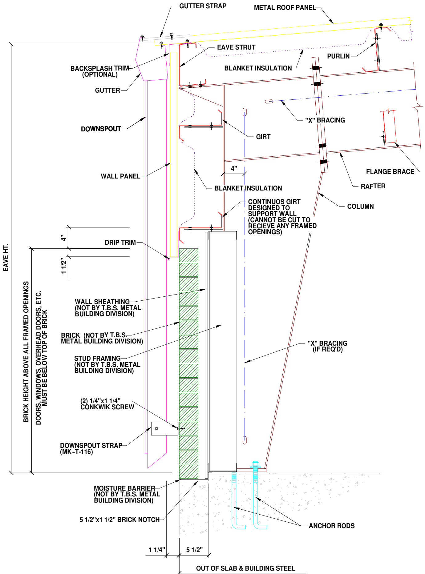
SIDEWALL SECTION AT PARTIAL BRICK WALL (BYPASS GIRTS SYSTEM REQUIRED)
