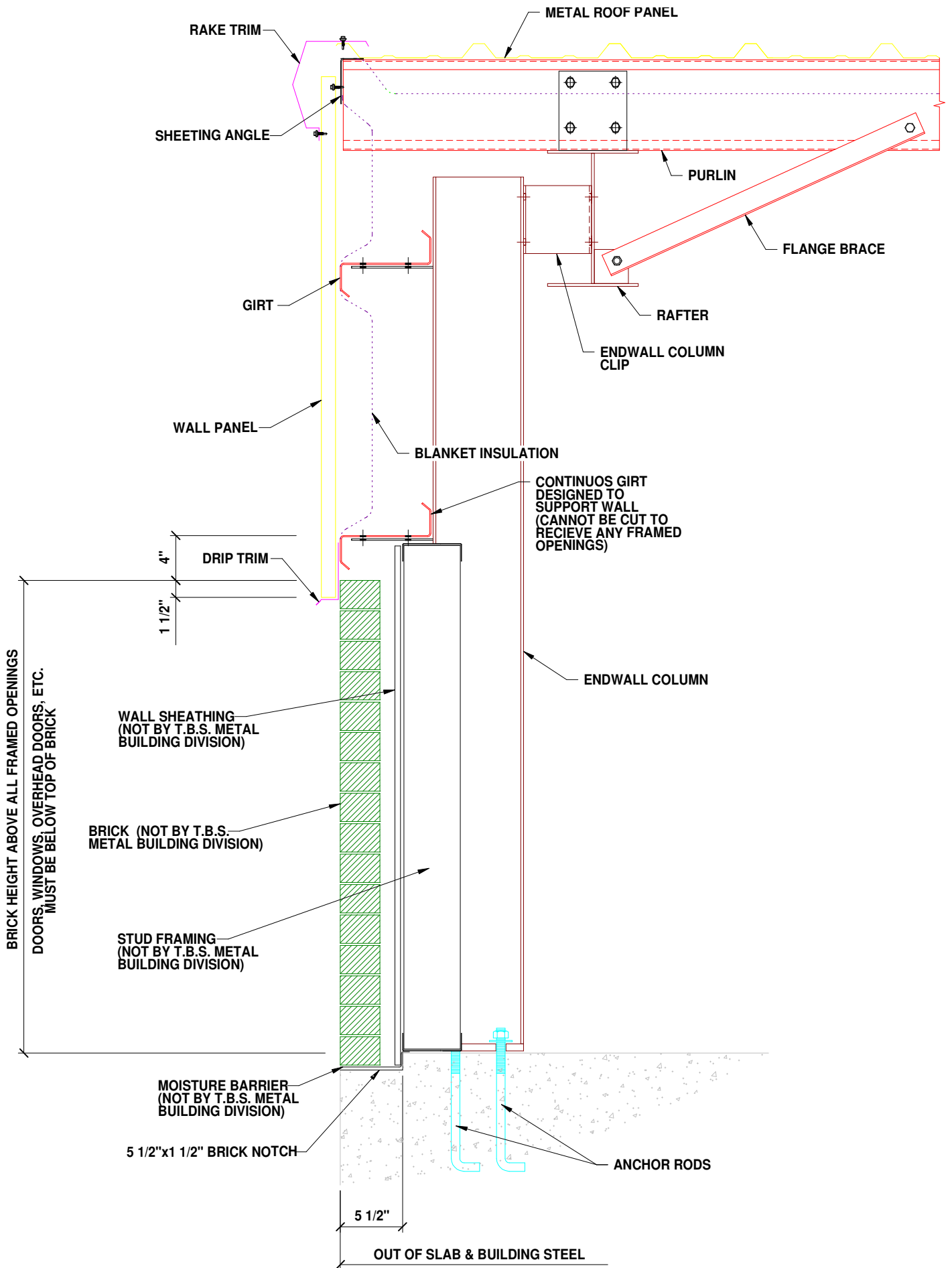
ENDWALL SECTION AT PARTIAL BRICK WALL (BYPASS GIRT SYSTEM REQUIRED)
